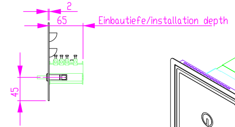
Schalterblende (optional lieferbar) switch panel - optional available
