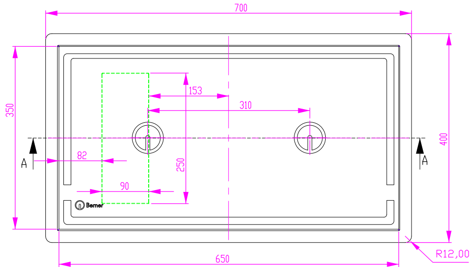
Ausschnitt in Abdeckung 680 x 380 cut out at cover panel
