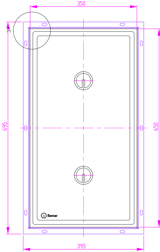
Ausschnitt in Abdeckung 356 x 656 cut out at cover panel
