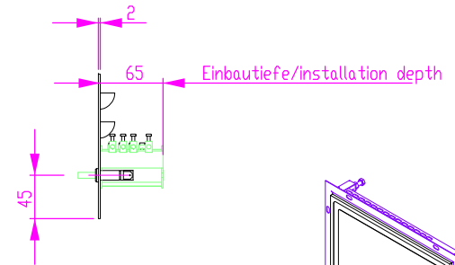
Schalterblende (optional lieferbar) switch panel - optional available
