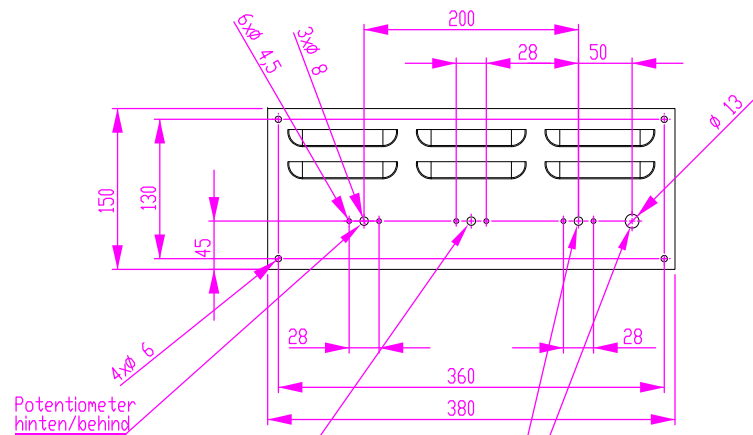
Schalterblende (optional lieferbar) switch panel - optional available
