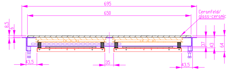
Ausschnitt in Abdeckung 356 x 656 cut out at cover panel
